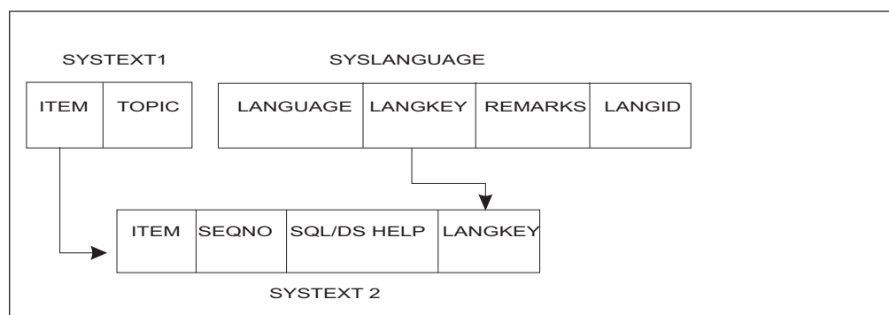
Figure 28. Relationships between SYSLANGUAGE, SYSTEXT1, and SYSTEXT2
