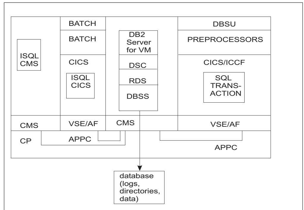
Figure 53. VSE Guest Sharing Configuration
