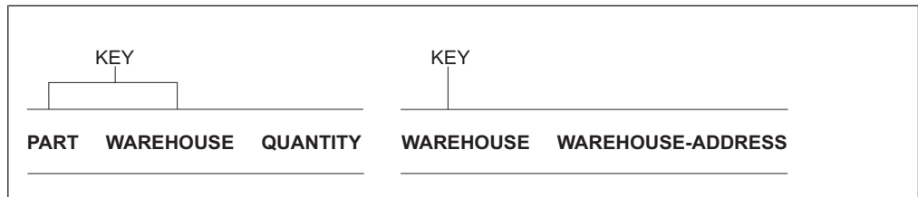
Figure 11. Two Tables Satisfy Second Normal Form
