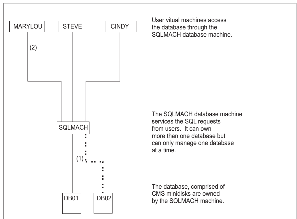
Figure 49. One Database Machine that Owns More than One Database
