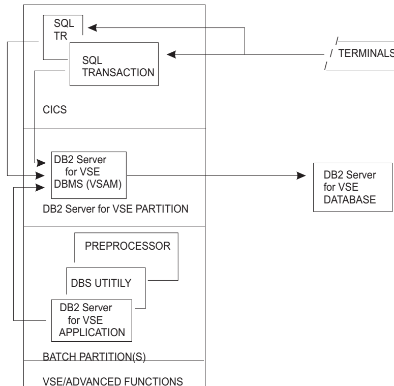
Figure 55. Online Transaction Processing Configuration
