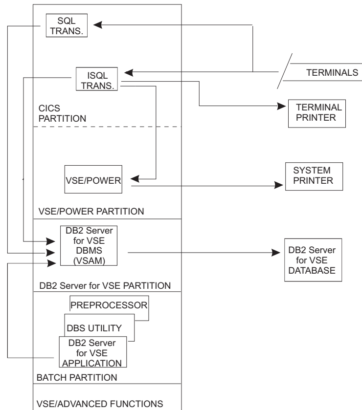
Figure 57. Query/Report Writing Configuration
