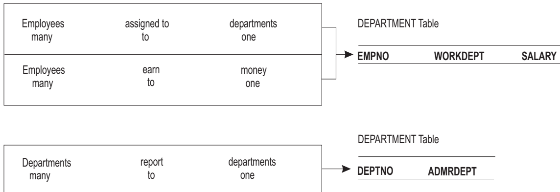
Figure 4. Assigning Many-to-One Facts to Tables
