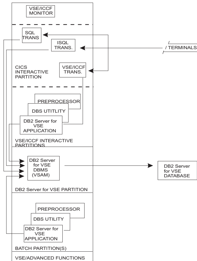
Figure 56. Application Development Configuration
