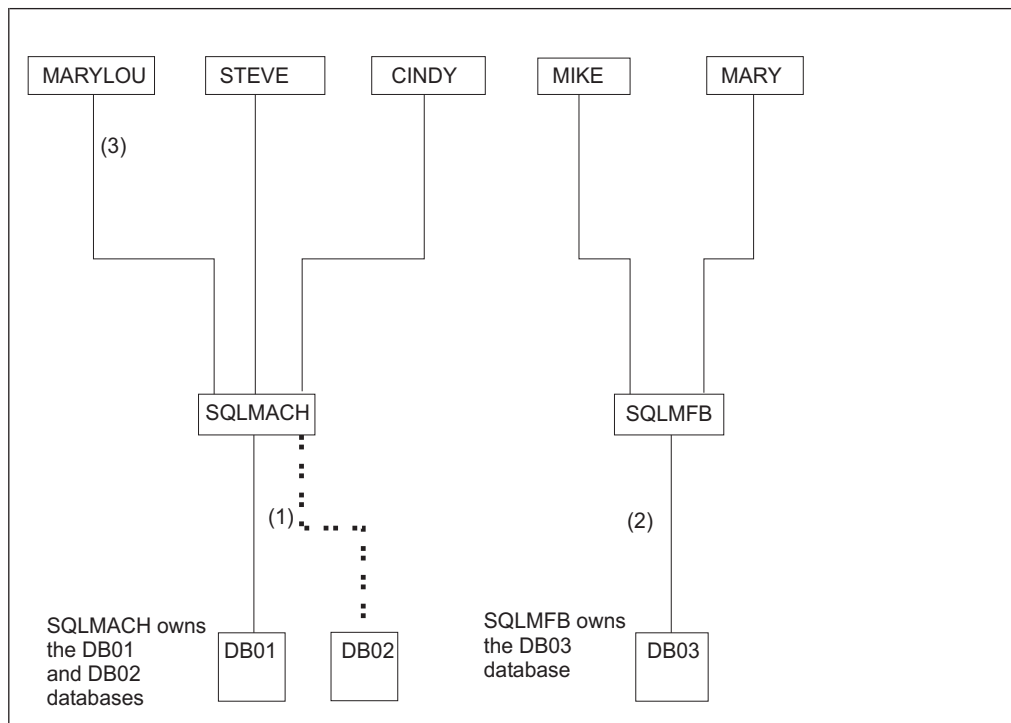
Figure 50. Two Database Machines with Three Databases
