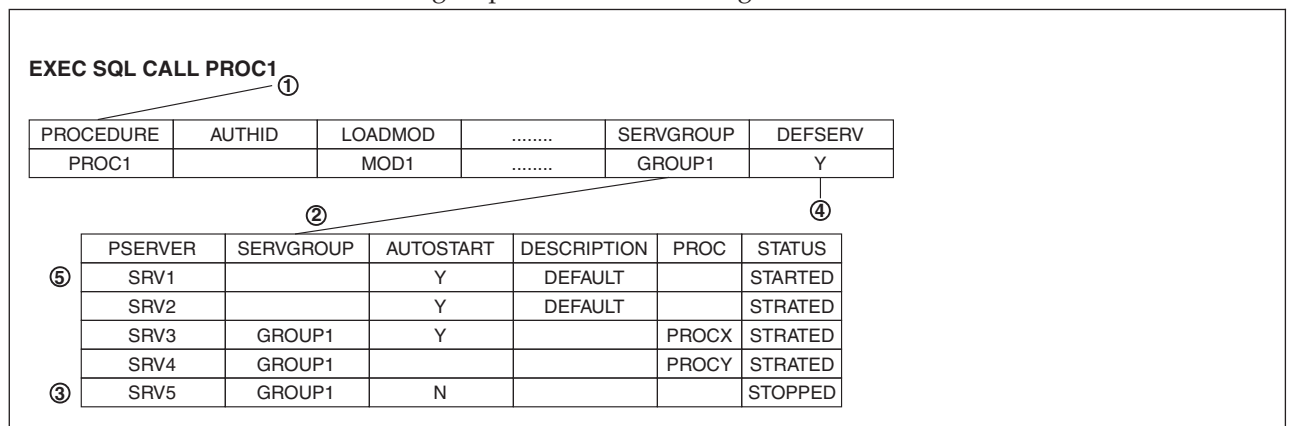
Figure 58. How DB2 Server for VSE & VM Determines the Stored Procedure Server to Use
