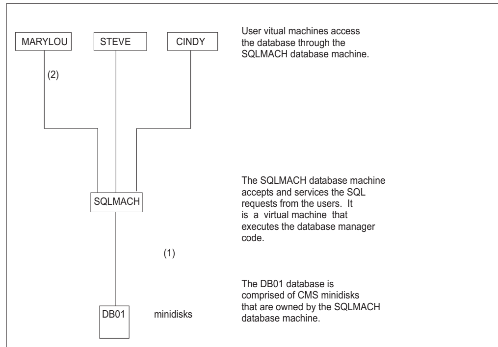
Figure 48. Example of One Database Machine Running One Database
