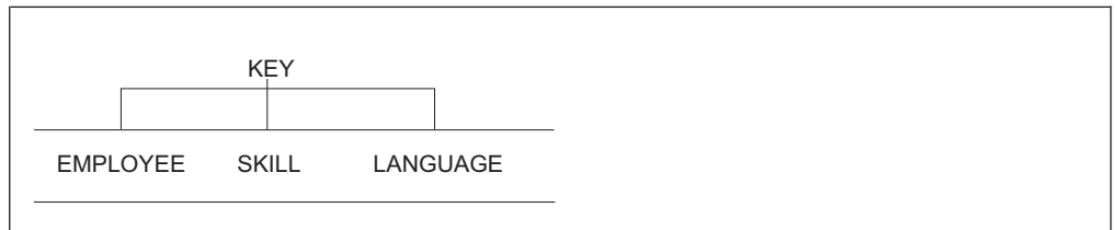
Figure 13. A Table That Violates Fourth Normal Form
