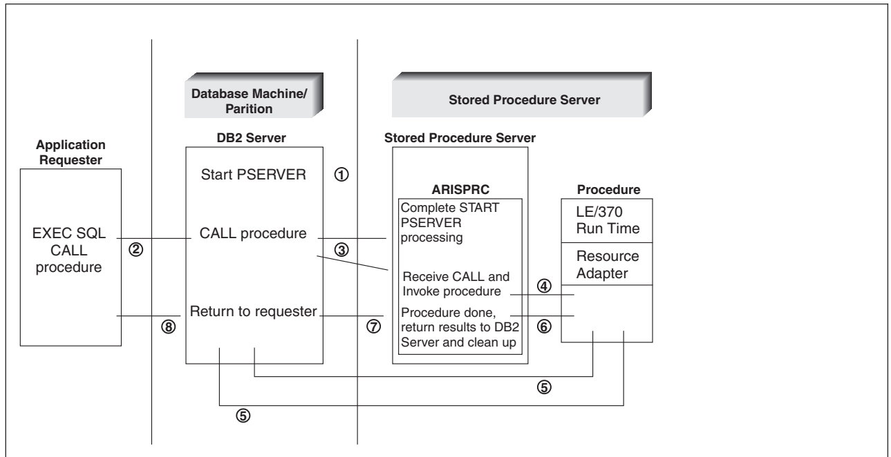
Figure 59. Stored Procedure Environment
