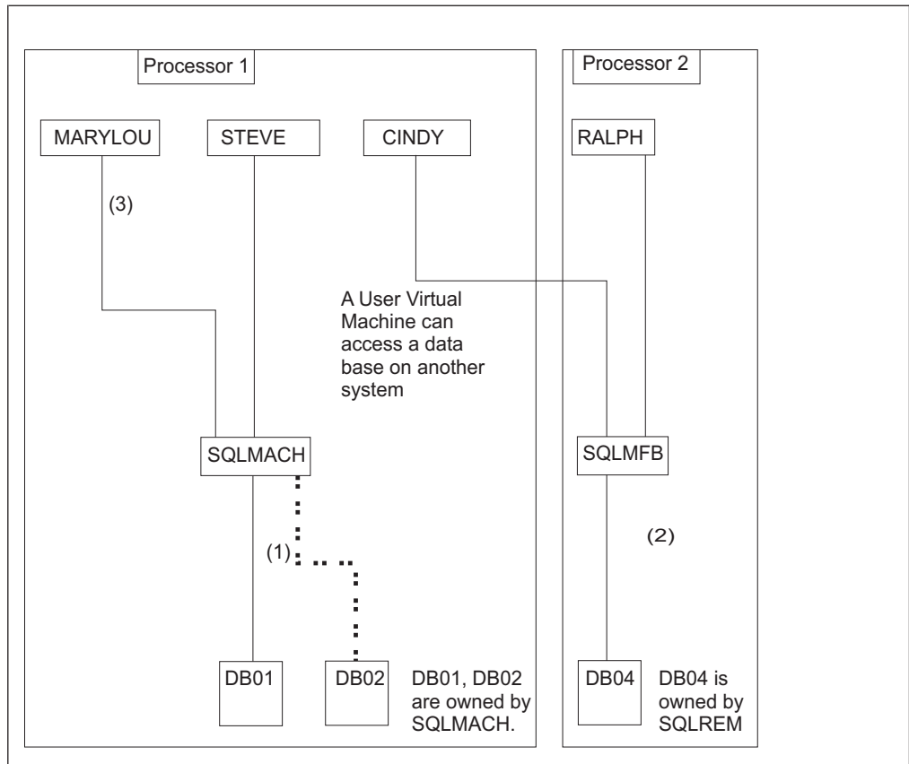
Figure 51. User Accessing a Database on Another Processor
